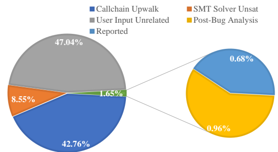
Fig. 6: The percentage of the UBs filtered out by each technique among the all UB instrumentations. If solely using SMT solver, only 8.55% UB instrumentation can be deemed false.
