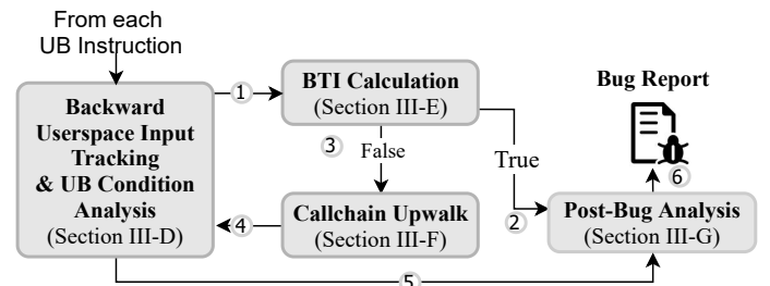
Fig. 2: KUBO workflow overview
