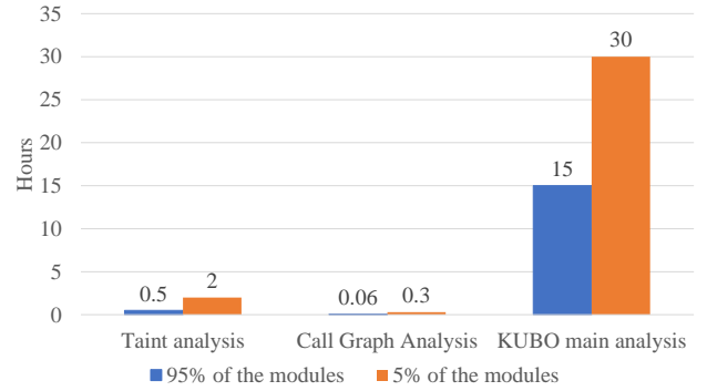
Fig. 8: Total time spent in each analysis phase. Although processing time varies between different modules due to their varying complexity, and all tasks were put into a thread pool, most of the modules can be finished within 16 hours(0.5h+4m+15h)(blue bar), a few extremely complex modules take much longer with the worse case scenario being 33 hours(2h+20m+30h)(red bar) detailed in § V-E.
